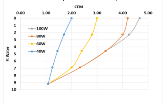
Flow vs water depth with different power
